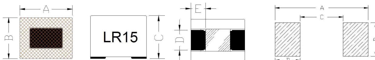
Dimension (Unit:mm):
